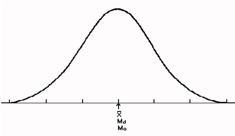
NORMAL
