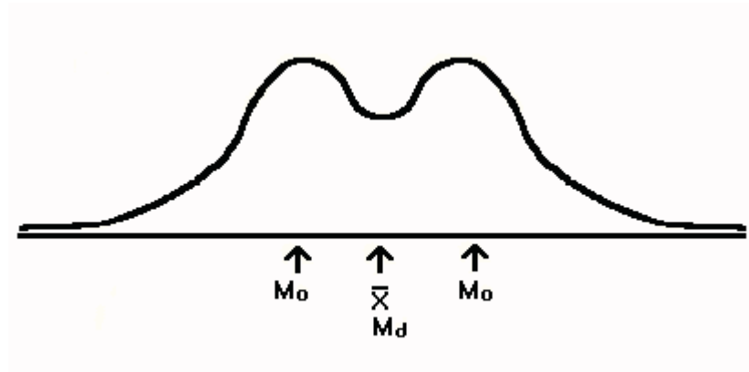
BIMODAL
